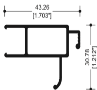
7112 VERTICAL MOSQUITERO
